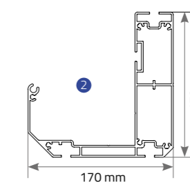
Extruded Frontal Gutter (Water-drain)
