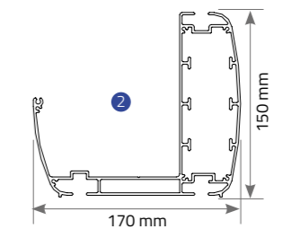
Extruded Frontal Gutter (Water-drain)
