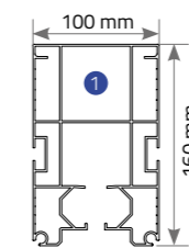
Rails
