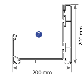
Extruded Frontal Gutter (Water-drain)
