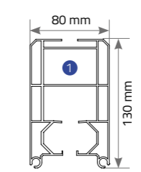
Rails
