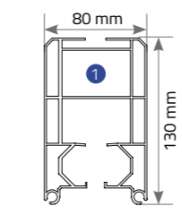
Rails
