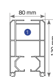
Rails
