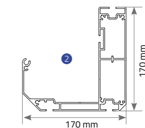
Extruded Frontal Gutter (Water-drain)
