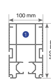
Rails
