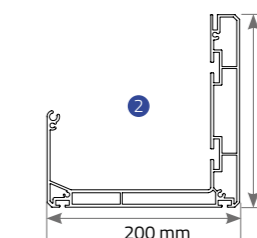
Extruded Frontal Gutter (Water-drain)
