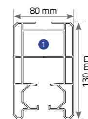
Rails
