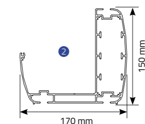
Extruded Frontal Gutter (Water-drain)
